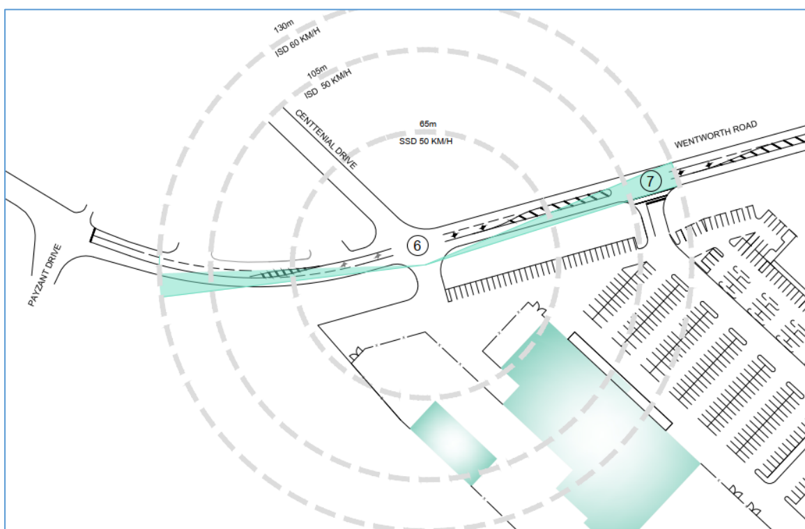
Figure 9 - Sight Distance for Driveway #6
