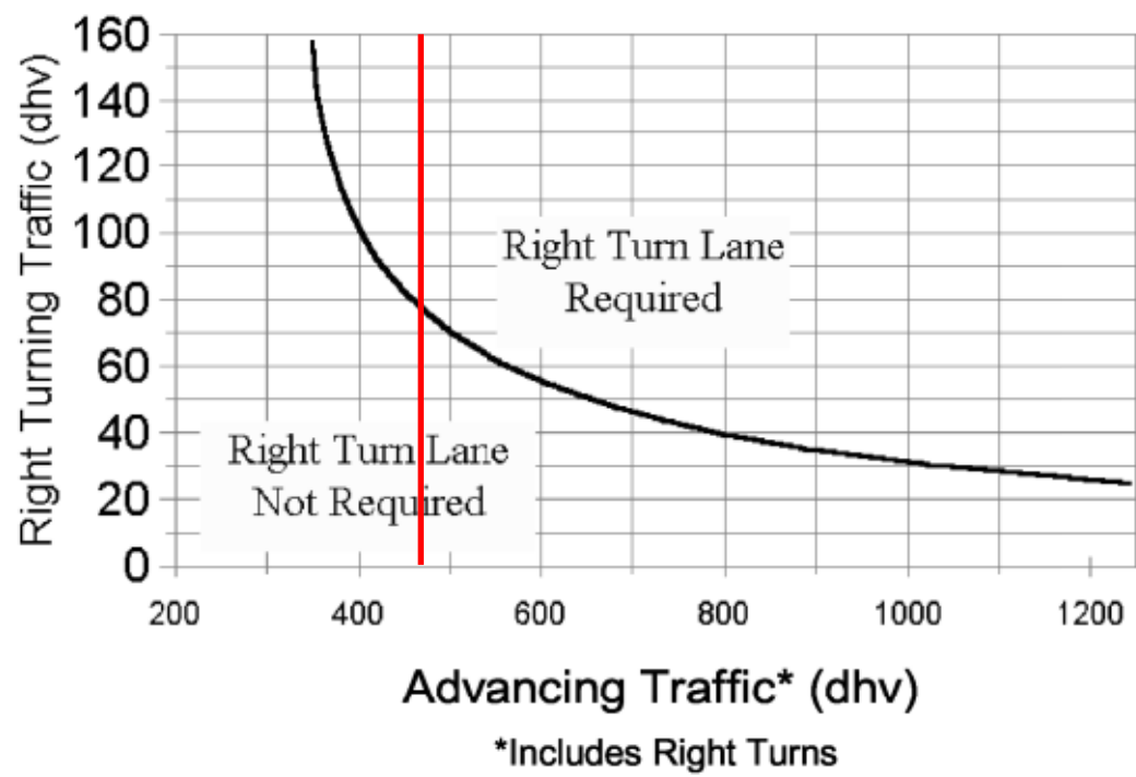
Figure 15 - Ohio DOT Right Turn Lane Warrant
