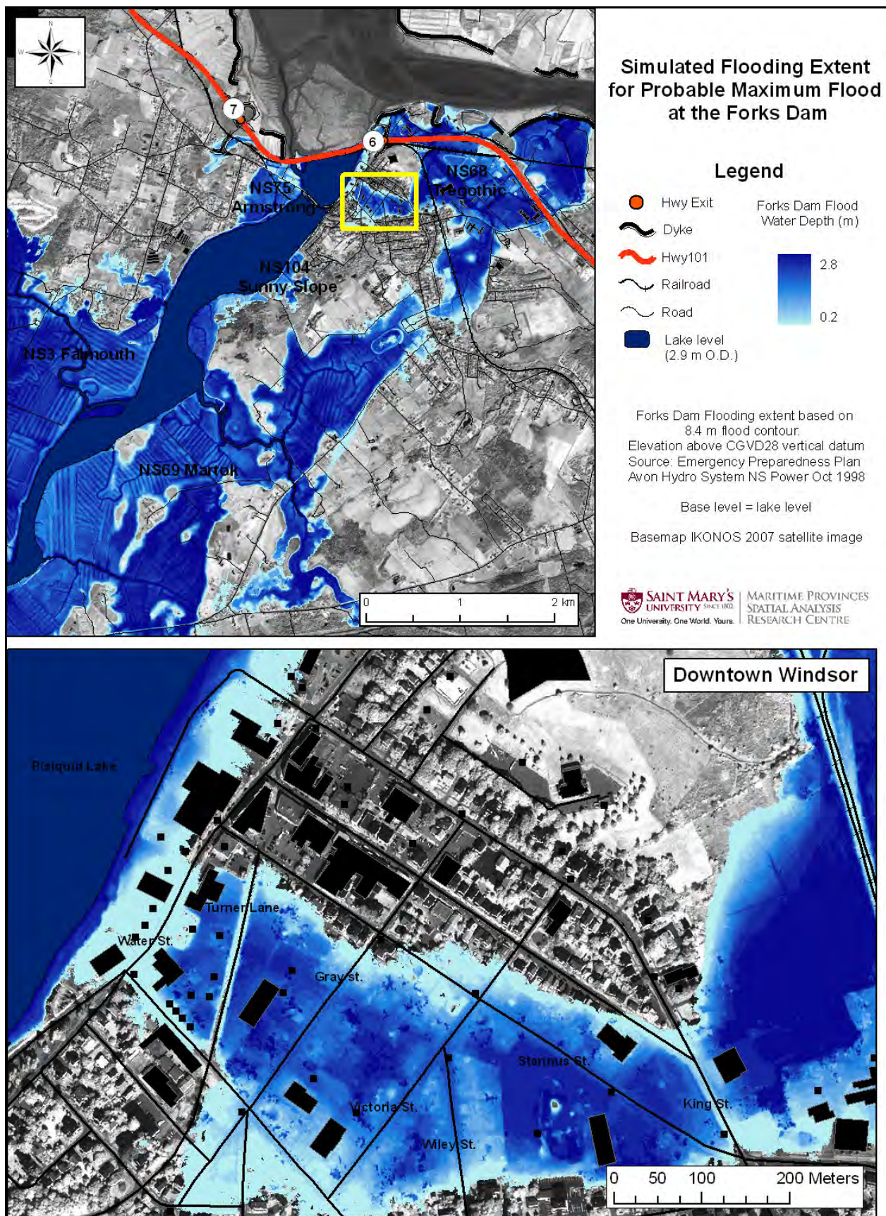
Figure 10: Simulated flood event for a probable maximum flood at the Forks Dam depicted damage to the Town of Windsor.
