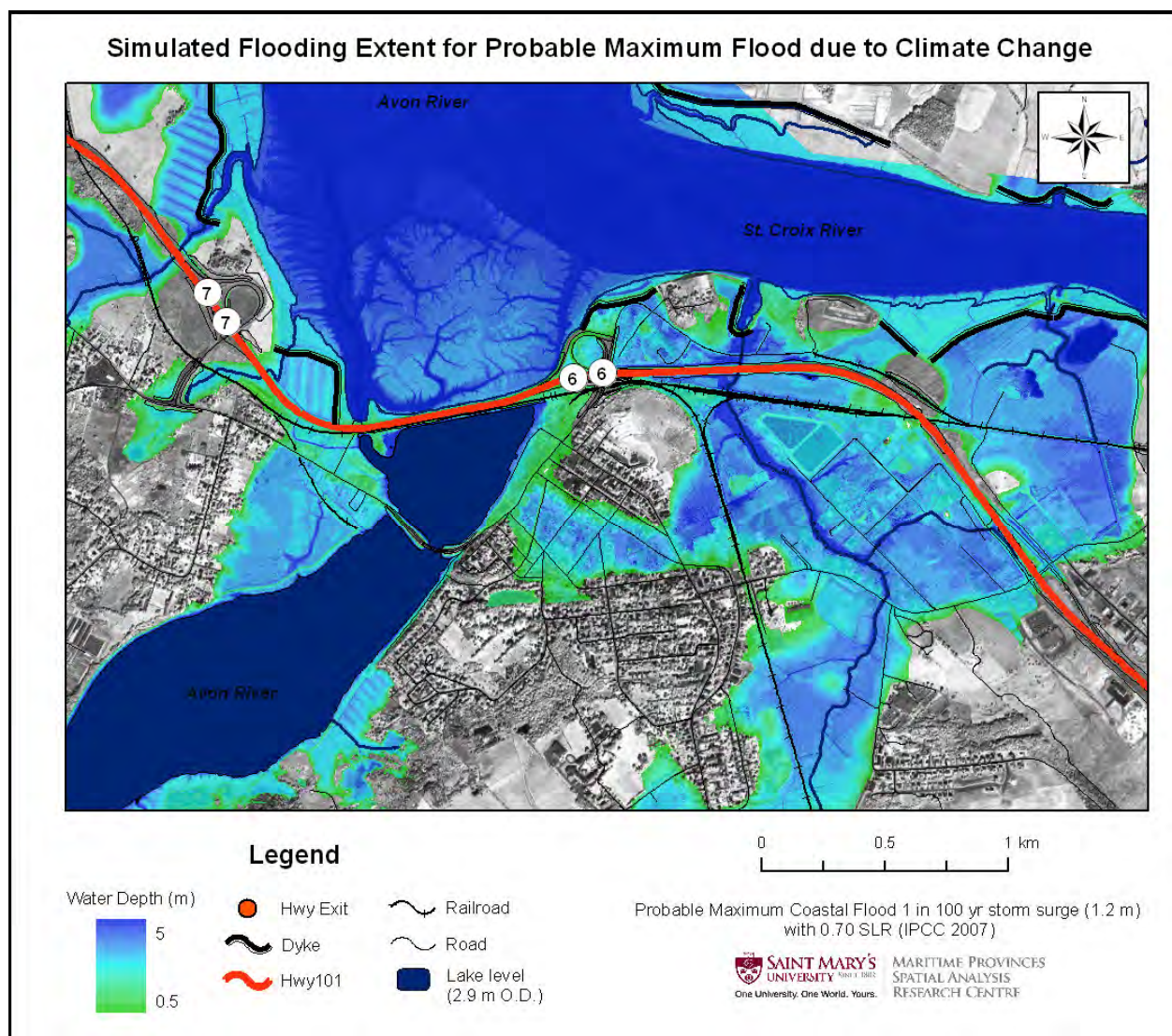
Figure 8: Simulated flooding extent and water depths for a 1 in 100 year storm surge (1.2 m) with a SLR of 0.7m.
