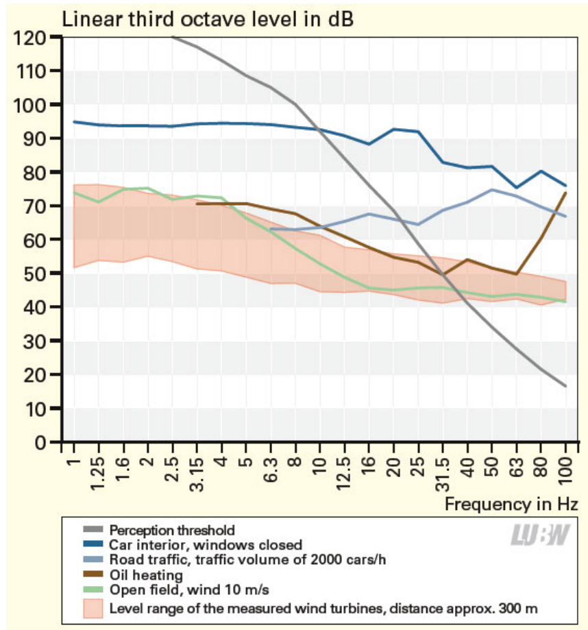
Figure 2. Measurements of infrasound and low frequency noise 300 m from wind turbines compared to other sources.
